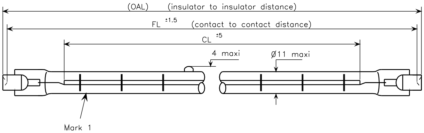
Fig. 1: Structure
